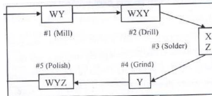
Group layout OR Cellular layout
